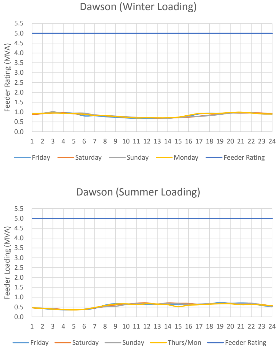
Figure 13. Winter and Summer Loadings on the Dawson Feeder
