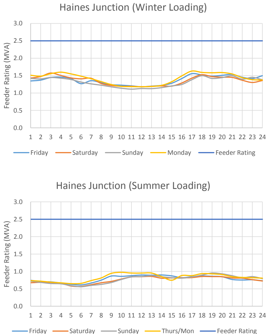
Figure 12. Winter and Summer Loadings on the Haines Junction Feeder
