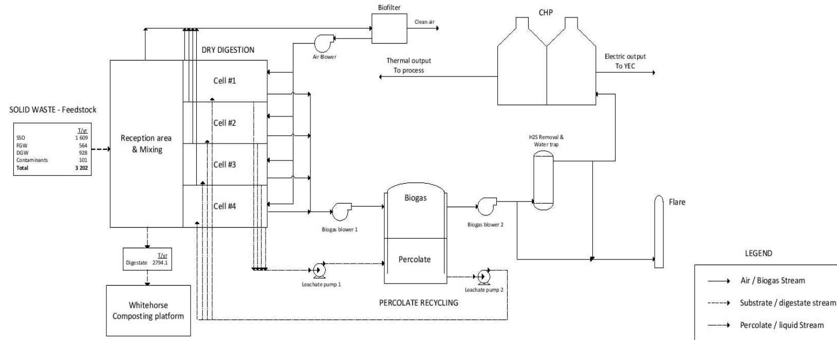
Figure 13 P&amp;ID
