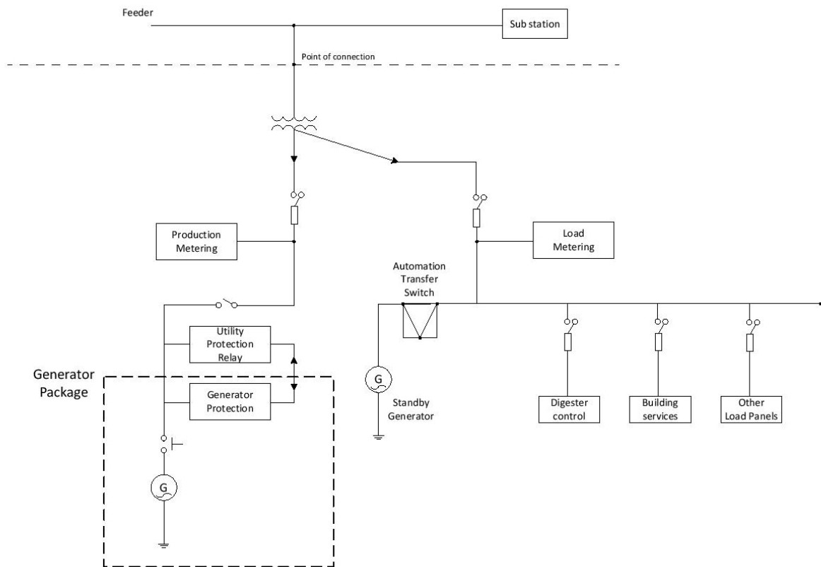
Figure 16 Electrical SLD
